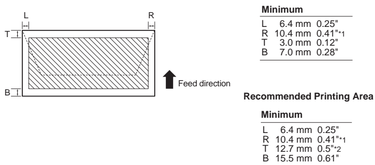
Figure 2-7 Printing Area (Envelope)
