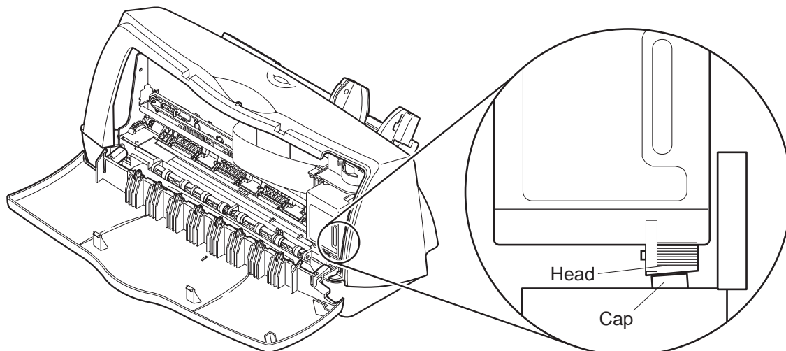
Figure 1-7 Capping Position
