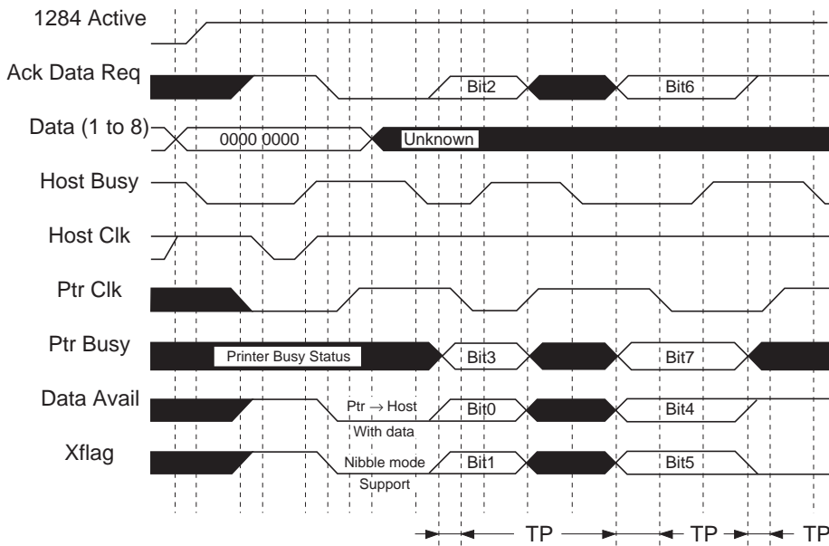
Figure 2-10 Timing Chart (Nibble Mode)
