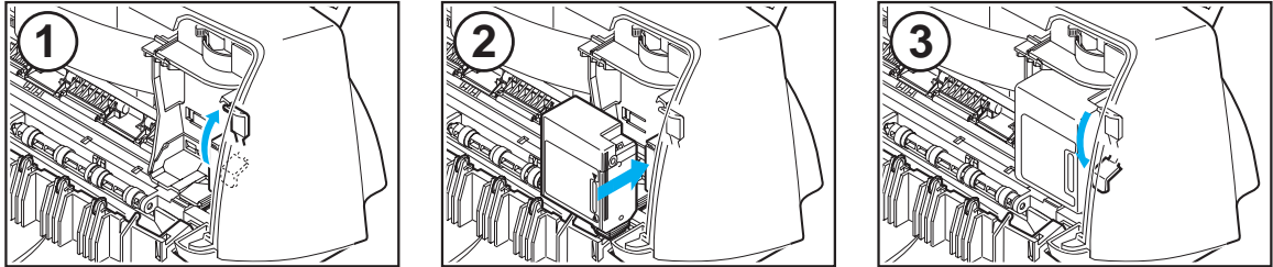
Figure 3-6 Cartridge Installation
