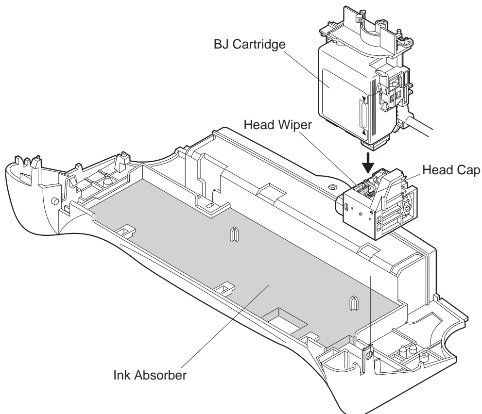
Figure 1-2 Ink Path
