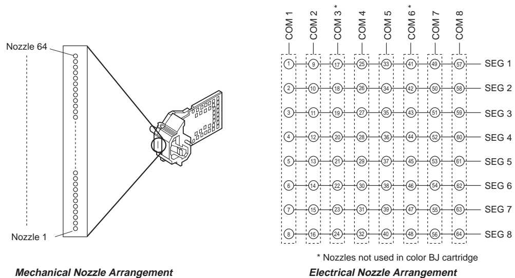
Figure 4-3 Nozzle Arrangement
