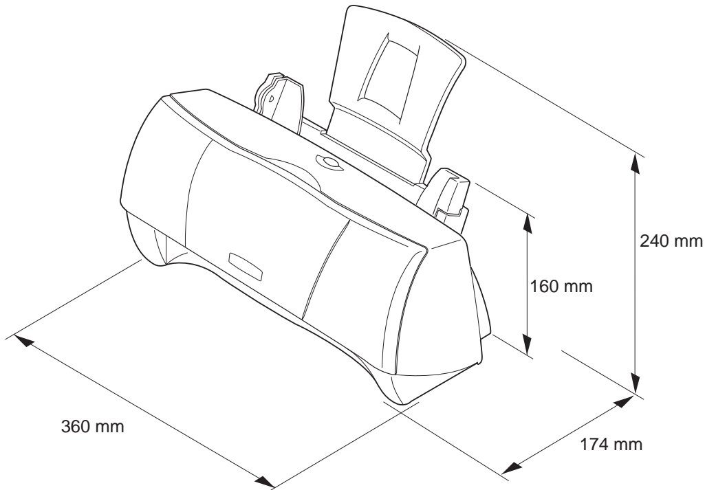
Figure 3-2 Printer Dimensions
