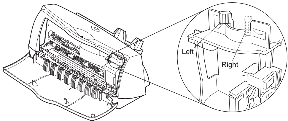
Figure 3-12 Paper Thickness Lever
