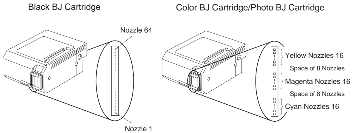
Figure 4-10 Nozzle Arrangement
