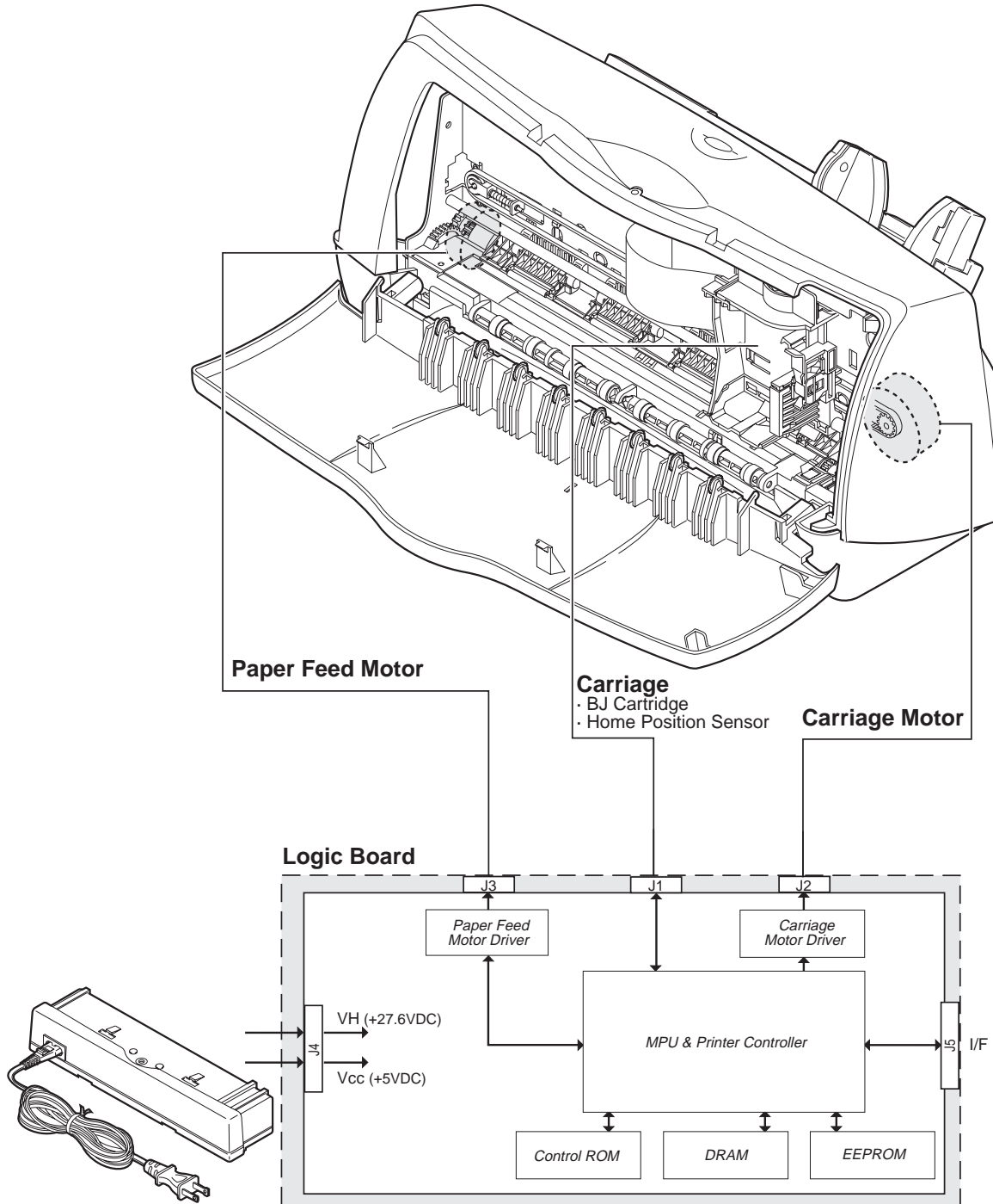
Figure 4-1 Block Diagram
