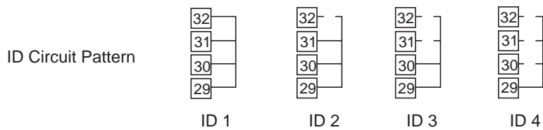
Figure 4-15 Head Rank ID
