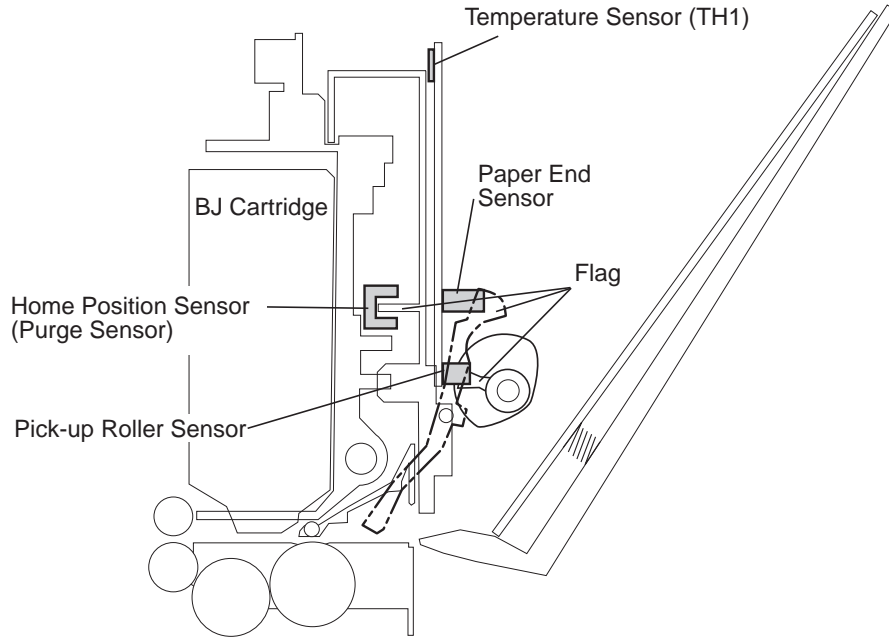
Figure 4-26 Sensors
